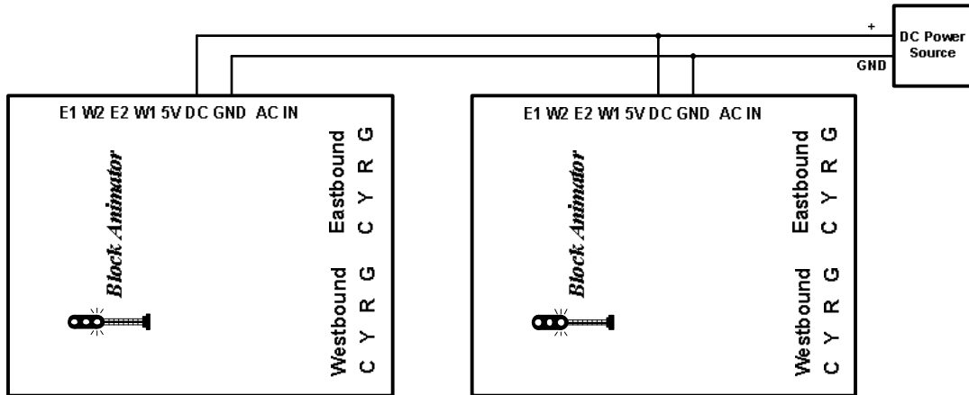
Figure 9 – DC power
