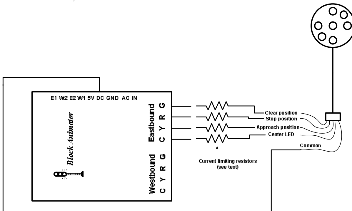
Figure 6 – LED-based (common cathode wiring) position light signals
