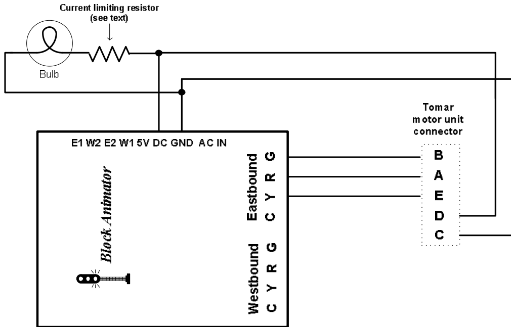
Figure 1 – Semaphore motor and signal
