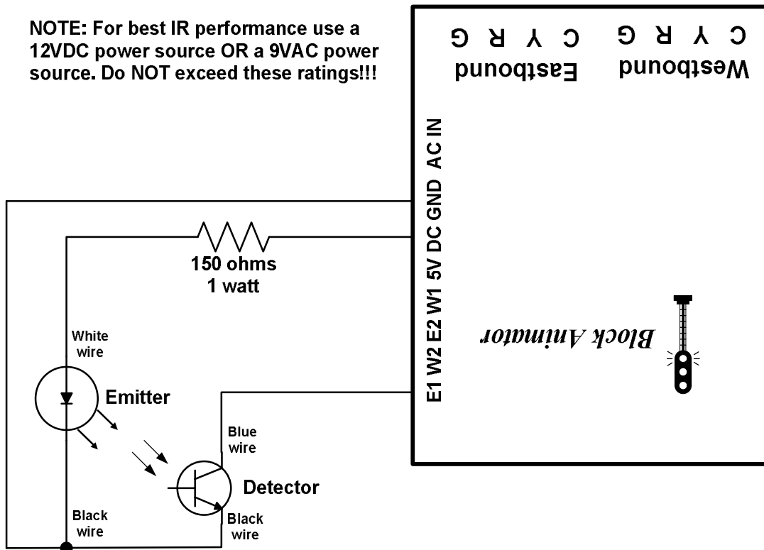
Figure 8 – IR component wiring
