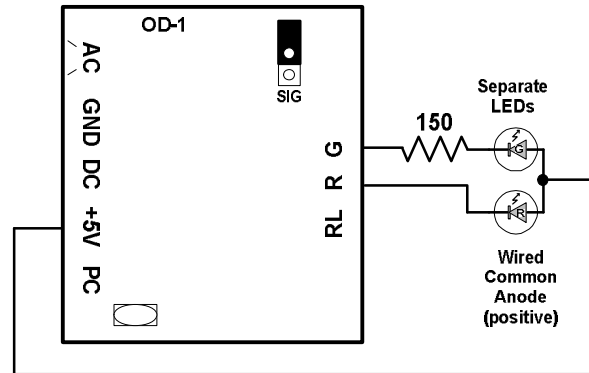
Figure 3 – Individual Red and Green LEDs (common anode)
