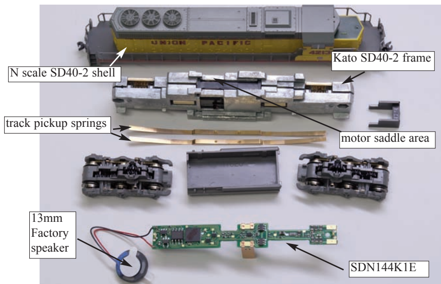
Figure 1: SDN144K1E installation in Kato N- SD40-2 frame preparation.
