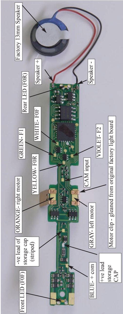
Figure 4: SDN144K1E: connections
