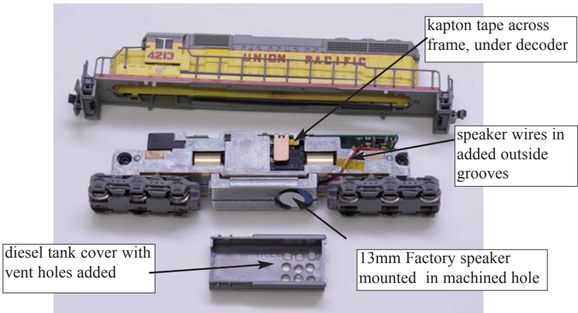
Figure 3: SDN144K1E Decoder installation in Kato SD40-2 - reassembled.
