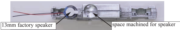
Figure 3: SDN144K1E Decoder installation in Kato SD40-2 - reassembled.
